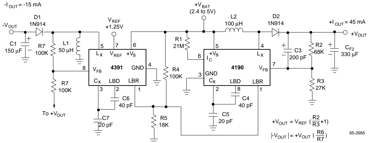
Figure 21. RC4190/RC4391 Power Supply ( \pm 15V )
