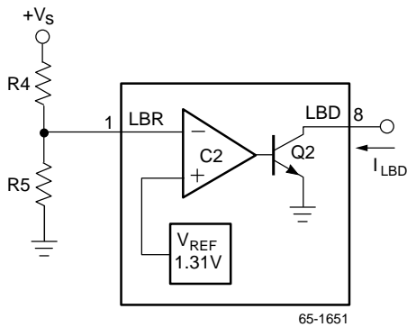
Figure 13. Low Battery Detector
